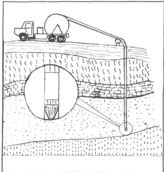
Fig. 2. Turbodrill on flexible drilling spring.
